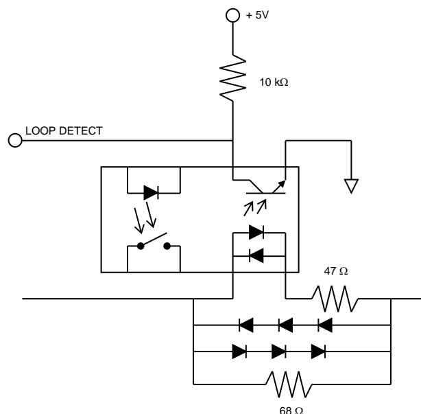
Figure 01: Loop Current Detection Circuit
