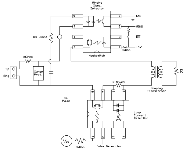
Figure 3: Application Using TR115
