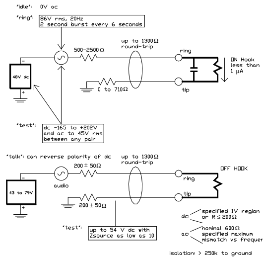
Figure 1: Telephone Line Basics
