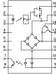
Figure 4: STS700 – Multi Function Relay
