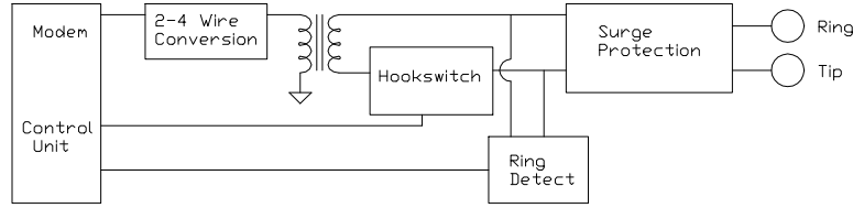
Figure 2: Typical Modem Circuit
