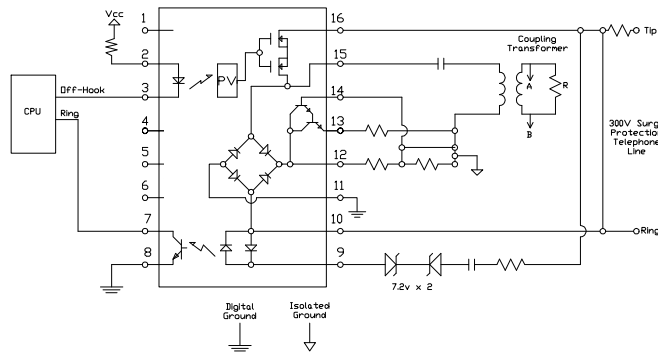
Figure 5: Sample Circuit Using STS700
